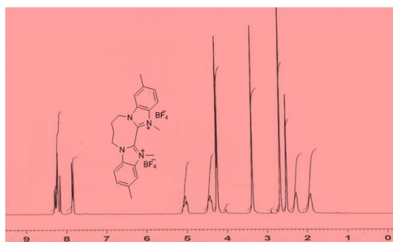
S25. 1 H-NMR spectrum of compound 7
