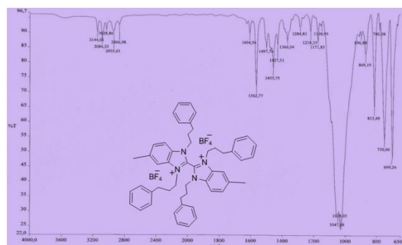
S8. IR spectrum of compound 2
