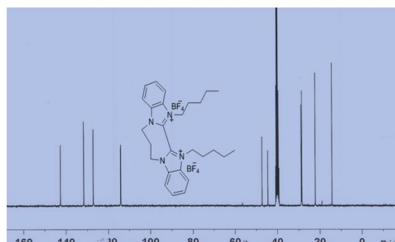
S18. 13 C-NMR spectrum of compound 5
