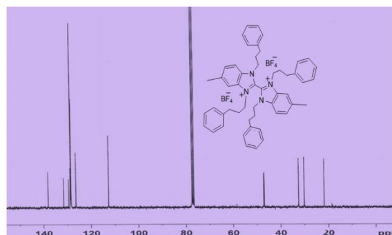
S6. 13 C-NMR spectrum of compound 2
