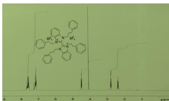
S9. 1 H-NMR spectrum of compound 3
