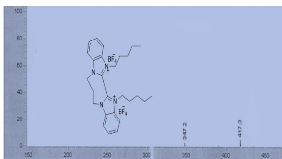
S19. LC-MS chromatogram of compound 5
