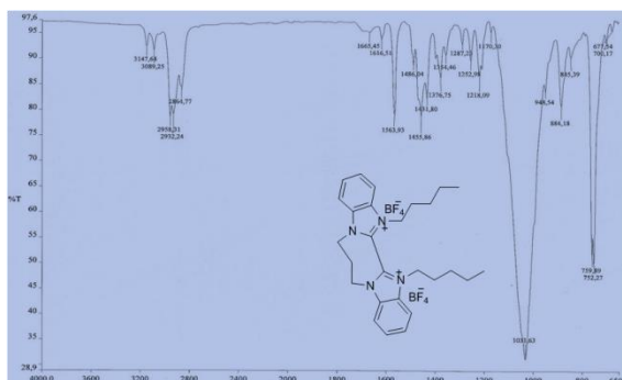
S20. IR spectrum of compound 5
