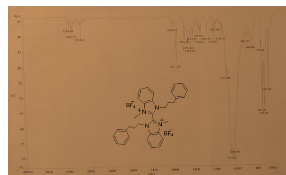
S16. IR spectrum of compound 4
