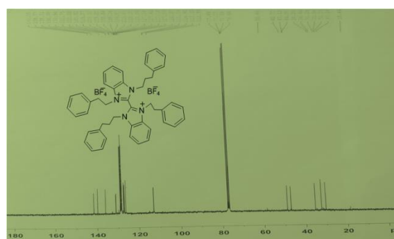
S10. 13 C-NMR spectrum of compound 3
