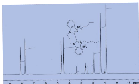
S17. 1 H-NMR spectrum of compound 5
