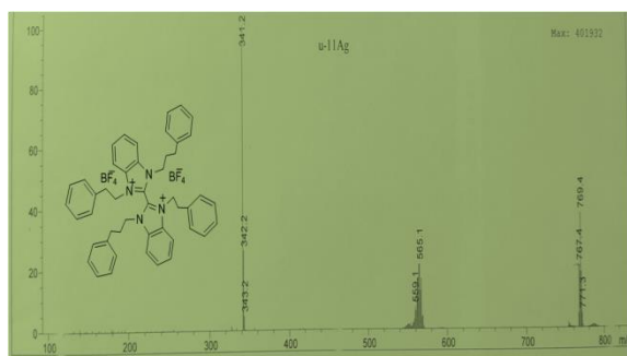
S11. LC-MS chromatogram of compound 3
