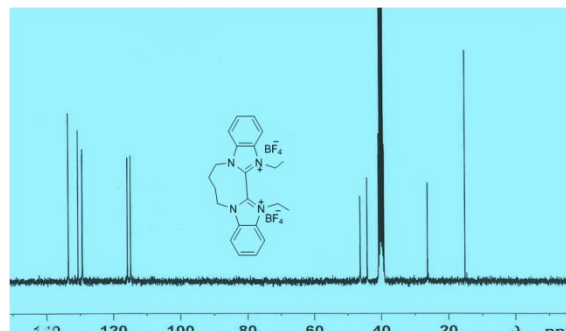
S22. 13 C-NMR spectrum of compound 6
