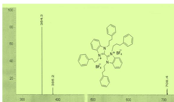
S3. LC-MS chromatogram of compound 1
