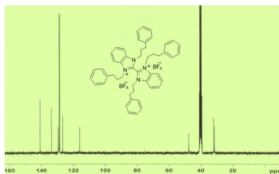
S2. ^{13}\text{C} -NMR spectrum of compound 1
