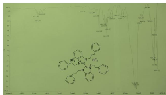
S12. IR spectrum of compound 3
