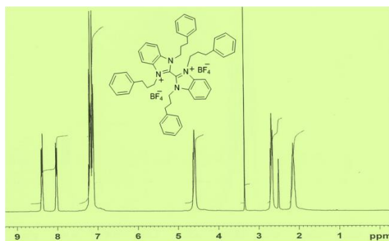
S1. ^1\text{H} -NMR spectrum of compound 1
