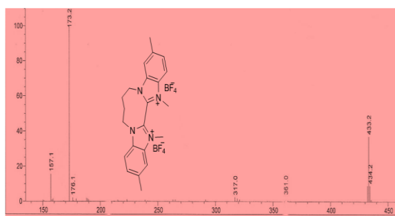
S27. LC-MS chromatogram of compound 7
