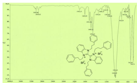
S4. IR spectrum of compound 1
