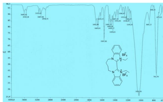
S24. IR spectrum of compound 6
