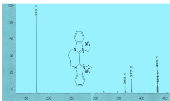
S23. LC-MS chromatogram of compound 6
