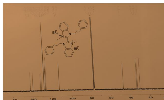
S14. 13 C-NMR spectrum of compound 4
