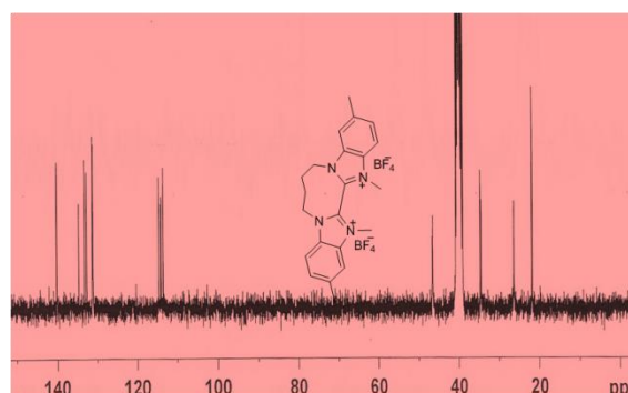
S26. 13 C-NMR spectrum of compound 7
