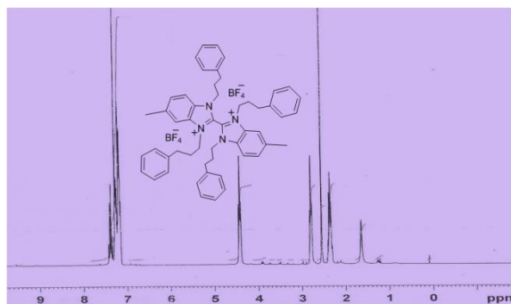
S5. 1 H-NMR spectrum of compound 2
