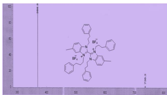
S7. LC-MS chromatogram of compound 2
