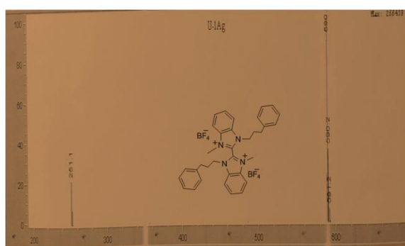
S15. LC-MS chromatogram of compound 4
