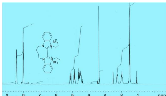
S21. 1 H-NMR spectrum of compound 6
