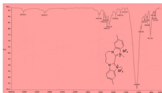
S28. IR spectrum of compound 7
