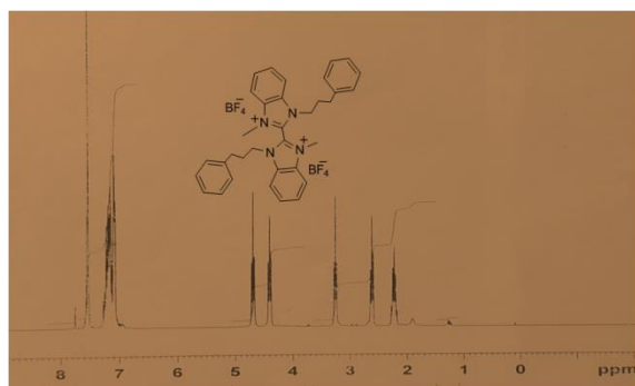
S13. 1 H-NMR spectrum of compound 4
