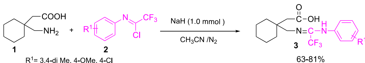
Scheme 2. Synthesis of 2-[1-({[2,2,2-trifluoro-1-(arylamino)ethylidene]amino)methyl)cyclohexyl]acetic acid derivatives ( 3a-c ).
