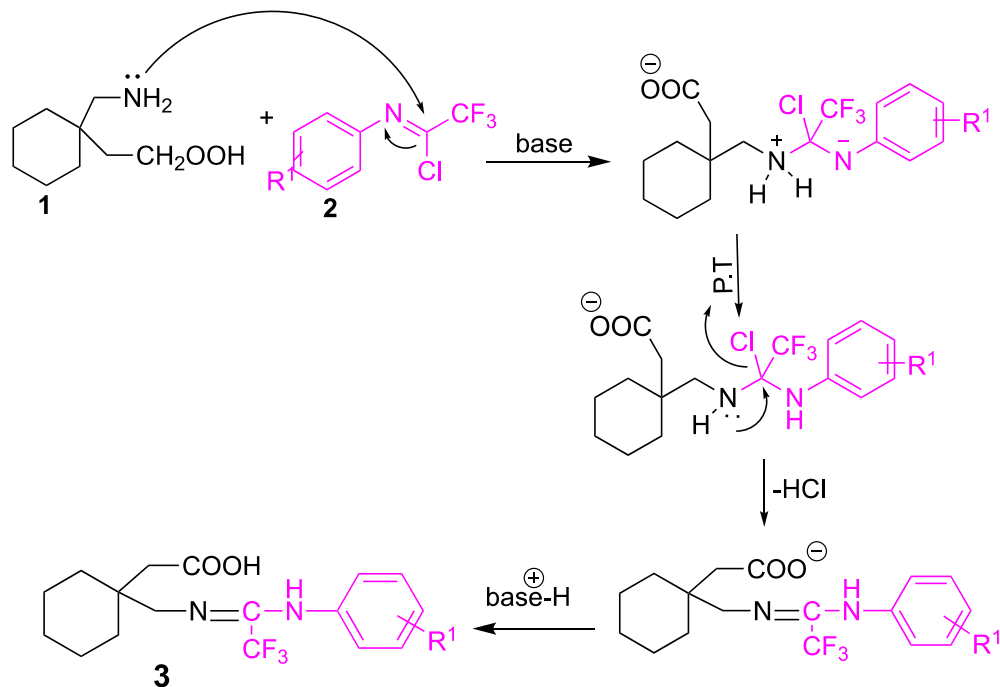
Scheme 3. A possible mechanism for the synthesis of 2-[1-({[2,2,2-trifluoro-1-(arylamino)ethylidene]amino}methyl)cyclohexyl]acetic acid derivatives.
