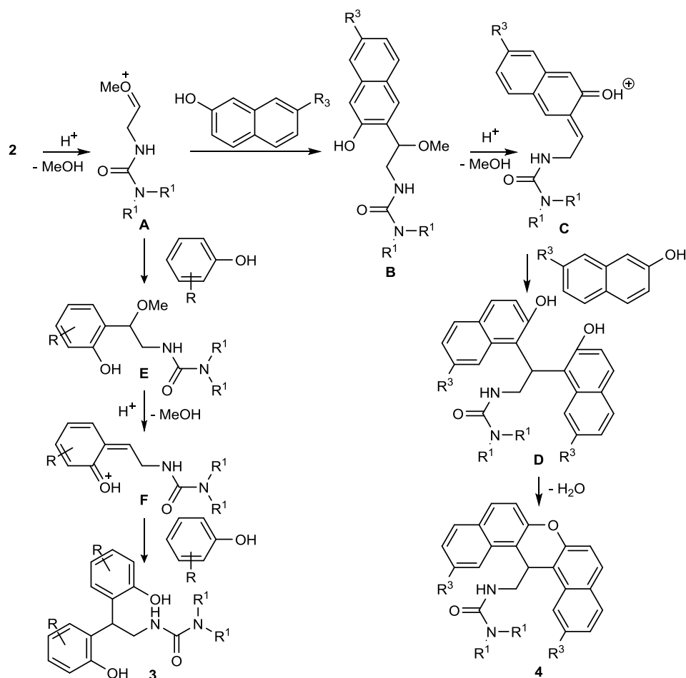
Scheme 3. Proposed mechanism for the substituted ureas 3,4 formation.
