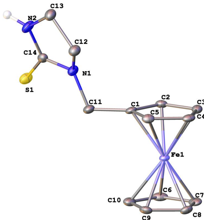
Figure 3. General view of molecule 7a presented in anisotropic displacement ellipsoids at 50% probability. Selected bond length and angles (Å and °): C1-C11 1.488(3), C11-N1 1.460(3), N1-C14 1.350(3), C14-N2 1.335(3), C14-S1 1.683(2), C1-C11-N1 112.21(19), N1-C14-S1 125.51(19), N1-C14-N2 109.0(2)
