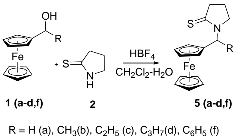
Scheme 1. Ferrocenylalkylation of pyrrolidine-2-thione 2 .
