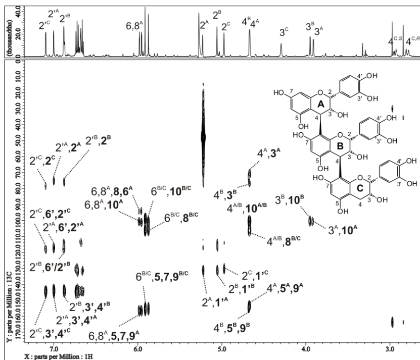
Figure S36. ^1\text{H} - ^{13}\text{C} -HMBC of compound 4 at -15^\circ\text{C} .
