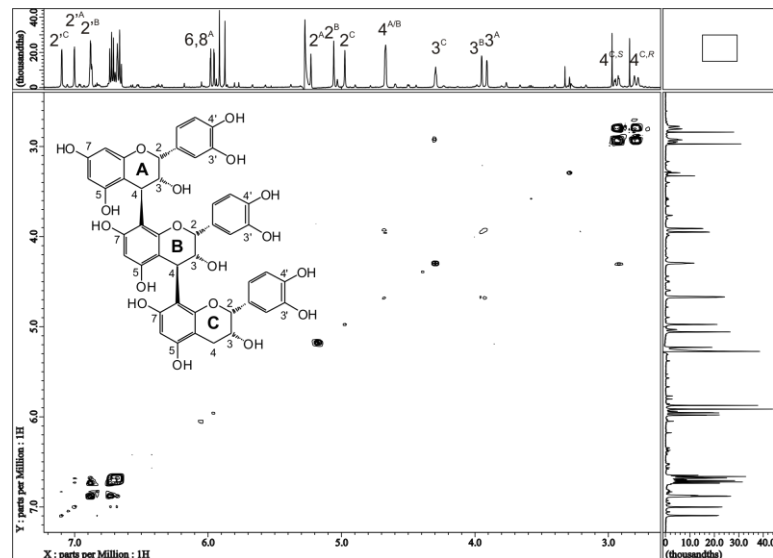
Figure S34. ^1\text{H} - ^1\text{H} -COSY of compound 4 at -15 °C.
