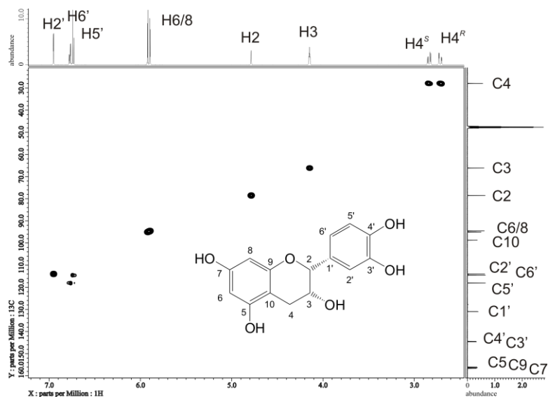
Figure S4. ^1\text{H} - ^{13}\text{C} -HMOC of compound 1b
