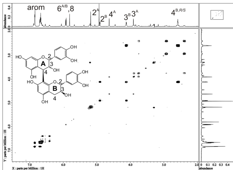
Figure S13. ^1\text{H} - ^1\text{H} -COSY of compound 2 at -15 °C
