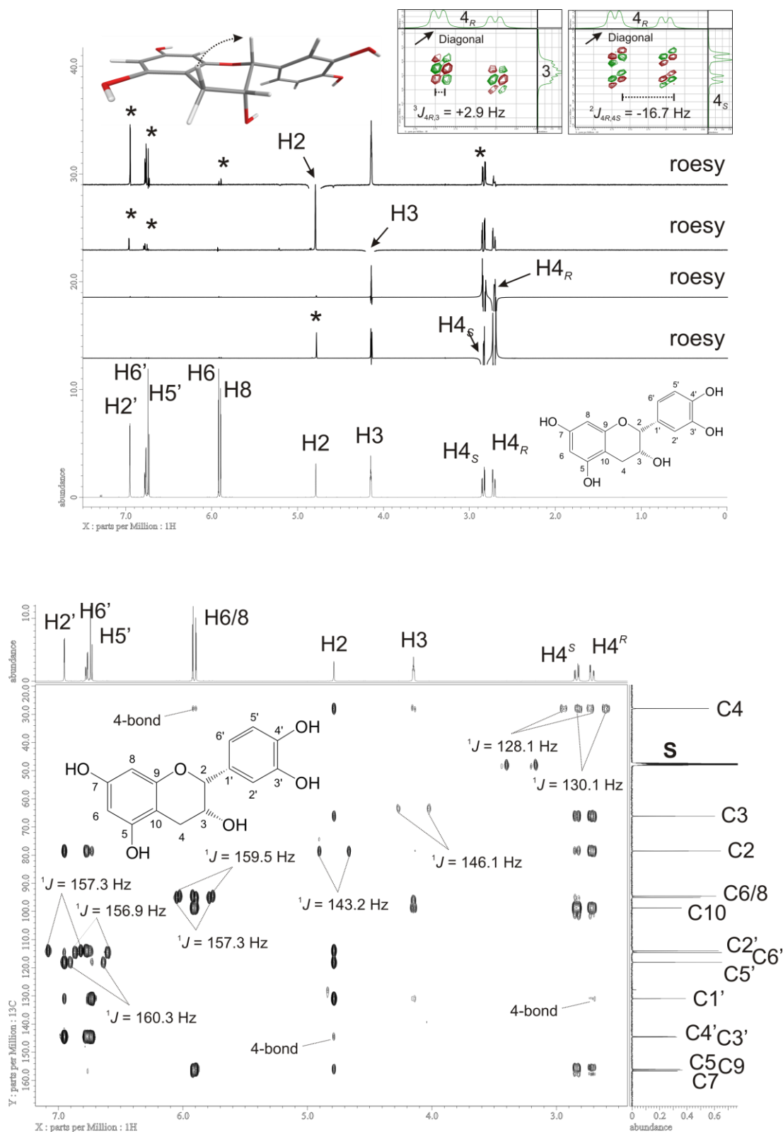
Figure S1. Top: Conformational analysis of (-)-1b. Small coupling constants of ^3J_{H4R,H3} = +4.6 Hz and ^3J_{H4S,H3} = +2.9 Hz (E-COSY, inset) as well as 1d-pfg-roesy response at H4 S and H2'/H6' upon irradiation of H2 confirmed the preferred tetrahydropyran- 2 H 3 conformation and conformational flexibility of the catechol; bottom: ^1\text{H} - ^{13}\text{C} -HMBC spectrum of (1b) with ^3J_{H3-C10} = 5.5 Hz, ^3J_{H4R-C2} = 0.4 Hz, and ^3J_{H4S-C2} = 5.3 Hz. Identities of all carbons were established from HMQC correlations and typical one-bond ^1\text{H} - ^{13}\text{C} -J-values were observed.
