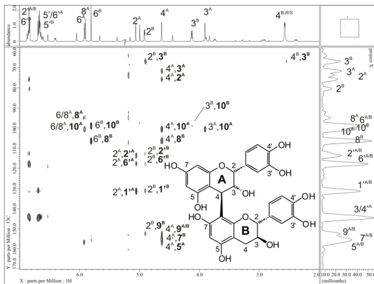
Figure S15. ^1\text{H} - ^{13}\text{C} -HMBC of compound 2 at -15 °C.
