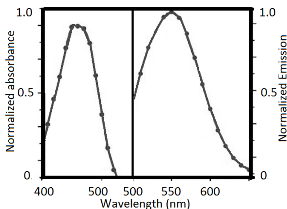
Figure 7. UV-visible spectrum (left) of 19b and its corresponding fluorescence spectrum (right) in acetonitrile; adapted from reference 24.
