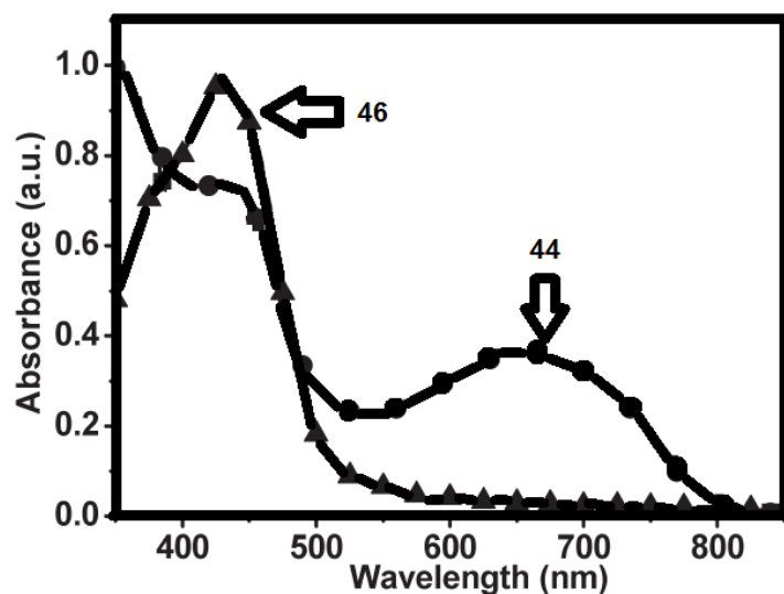
Figure 15. UV-visible spectra of polymer films of 44 and 46 on a quartz plate; adapted from reference 12.
