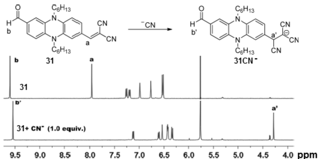
Figure 13. 1 H NMR spectrum of 31 in CD 2 Cl 2 (top) and after addition of 1.0 equiv. of cyanide anion (bottom); adapted from reference 29.
