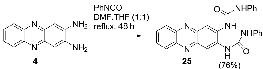
Scheme 8. Synthesis of 1-Phenyl-3-[3-(3-phenylureido)-phenazin-2-yl]-urea based anion sensor.
