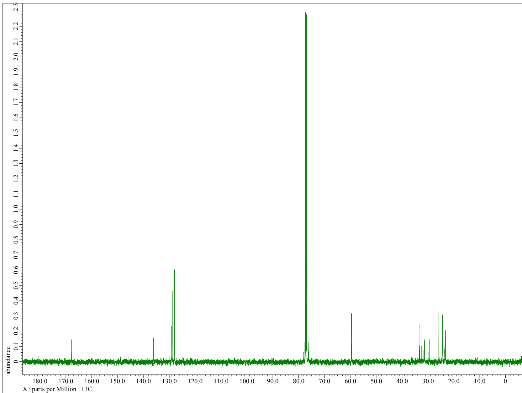
^{13}\text{C} NMR of Compound 32a+b [( \pm )-(trans-2-(cyclohexyloxy)cyclohexyl 2-chloro-2-phenylethanoate]
