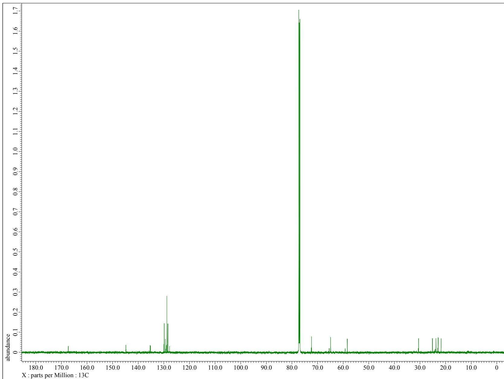
^{13}\text{C} NMR of Compound 33a+b [( \pm )-( trans -2-( p -tolylsulfonyl)cyclohexyl 2-chloro-2-phenylethanoate]
