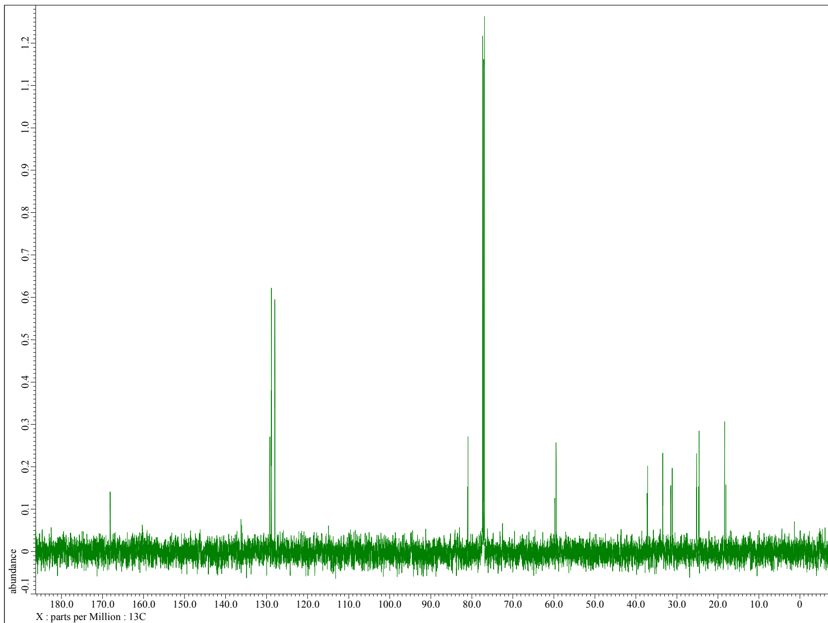
^{13}\text{C} NMR of Compound 34a+b [( \pm )- trans -2-(methyl)cyclohexyl 2-chloro-2-phenylethanoate]
