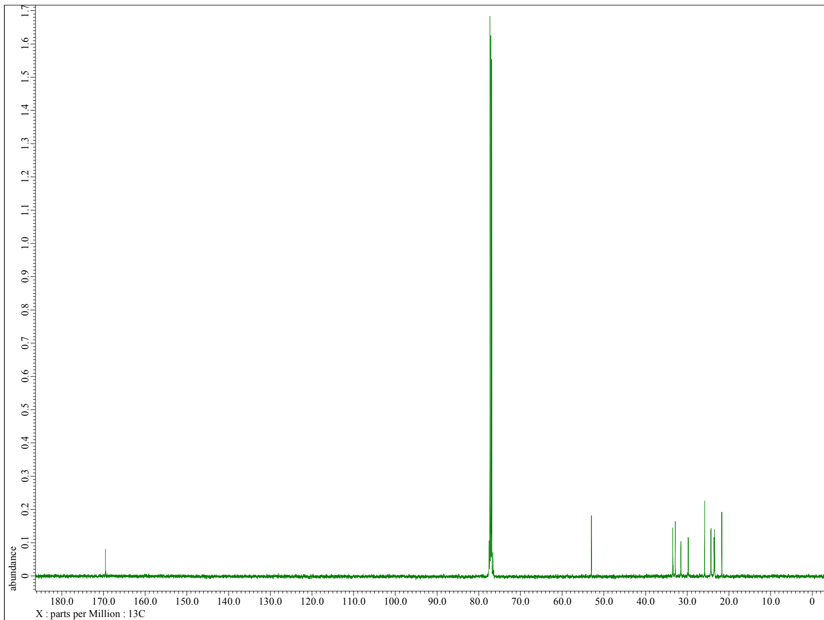
^{13}\text{C} NMR of Compound 23a+b [( \pm )-( trans -2-(cyclohexyloxy)cyclohexyl 2-chloropropanoate)]
