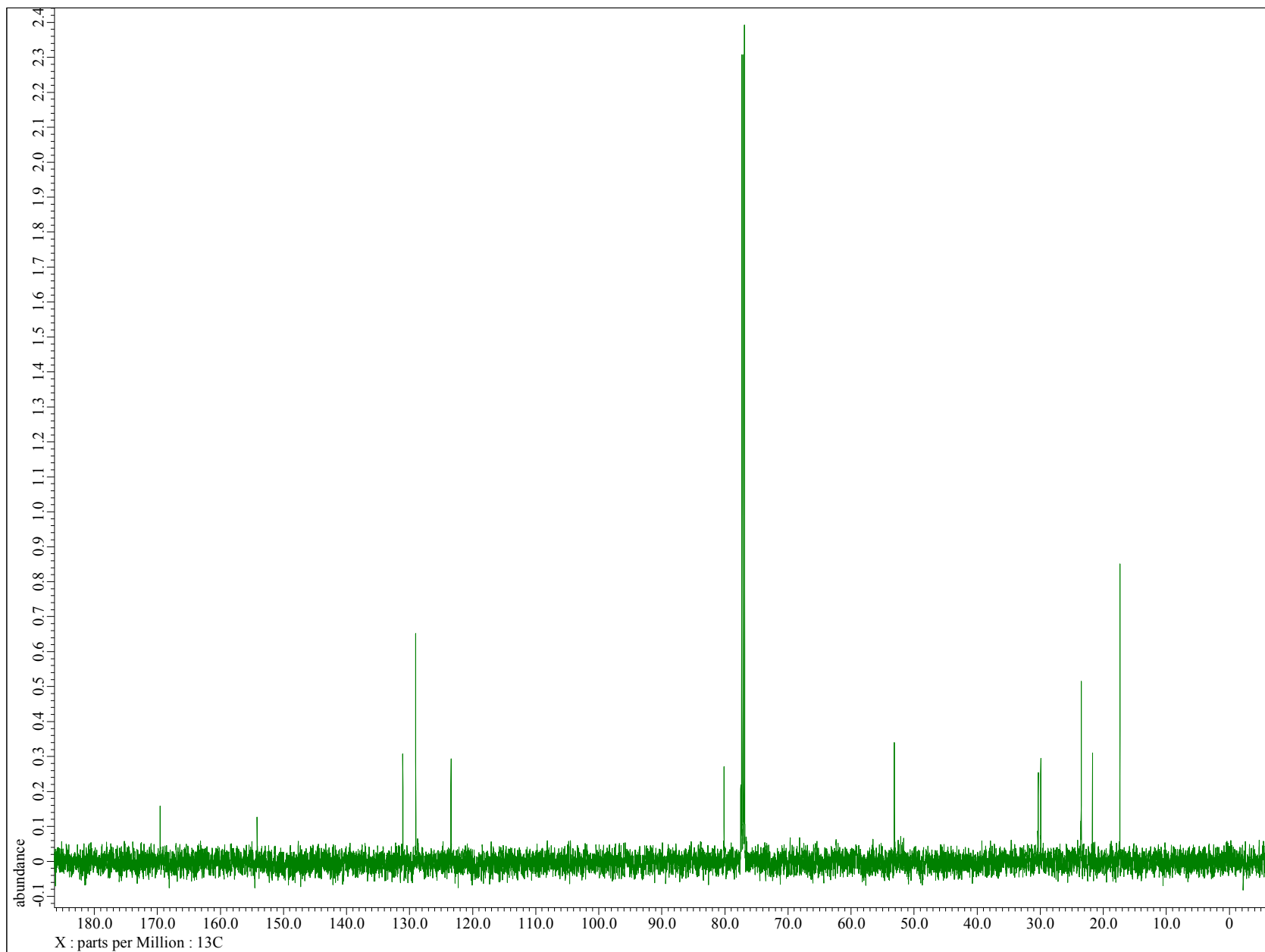
^{13}\text{C} NMR of Compound 22a+b [( \pm )-(trans-2-(2,6-dimethylphenoxy)cyclohexyl 2-chloropropanoate]
