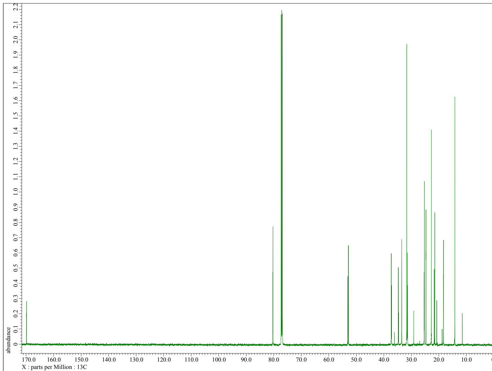
^{13}\text{C} NMR of Compound 28a+b [( \pm )-(trans-2-methylcyclohexyl) 2-chloropropanoate]
