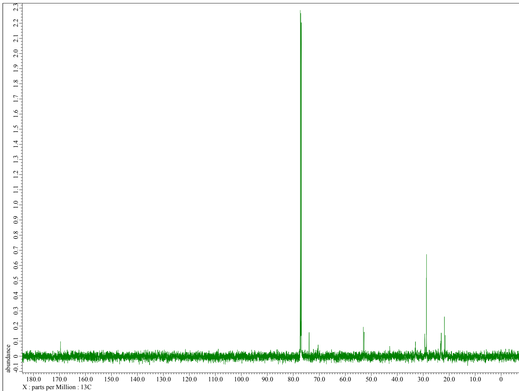
^{13}\text{C} NMR of Compound 24a+b [( \pm )-( trans -2-( tert -butoxy)cyclohexyl 2-chloropropanoate]
