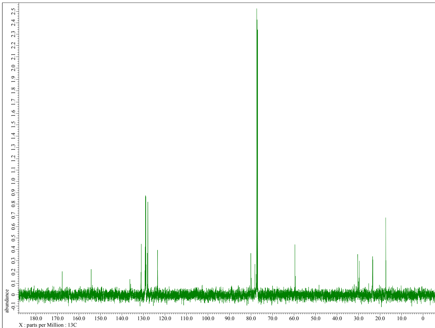
13 C NMR of Compound 31a+b [(±)-(trans-2-(2,6-dimethylphenoxy)cyclohexyl 2-chloro-2-phenylethanoate]
