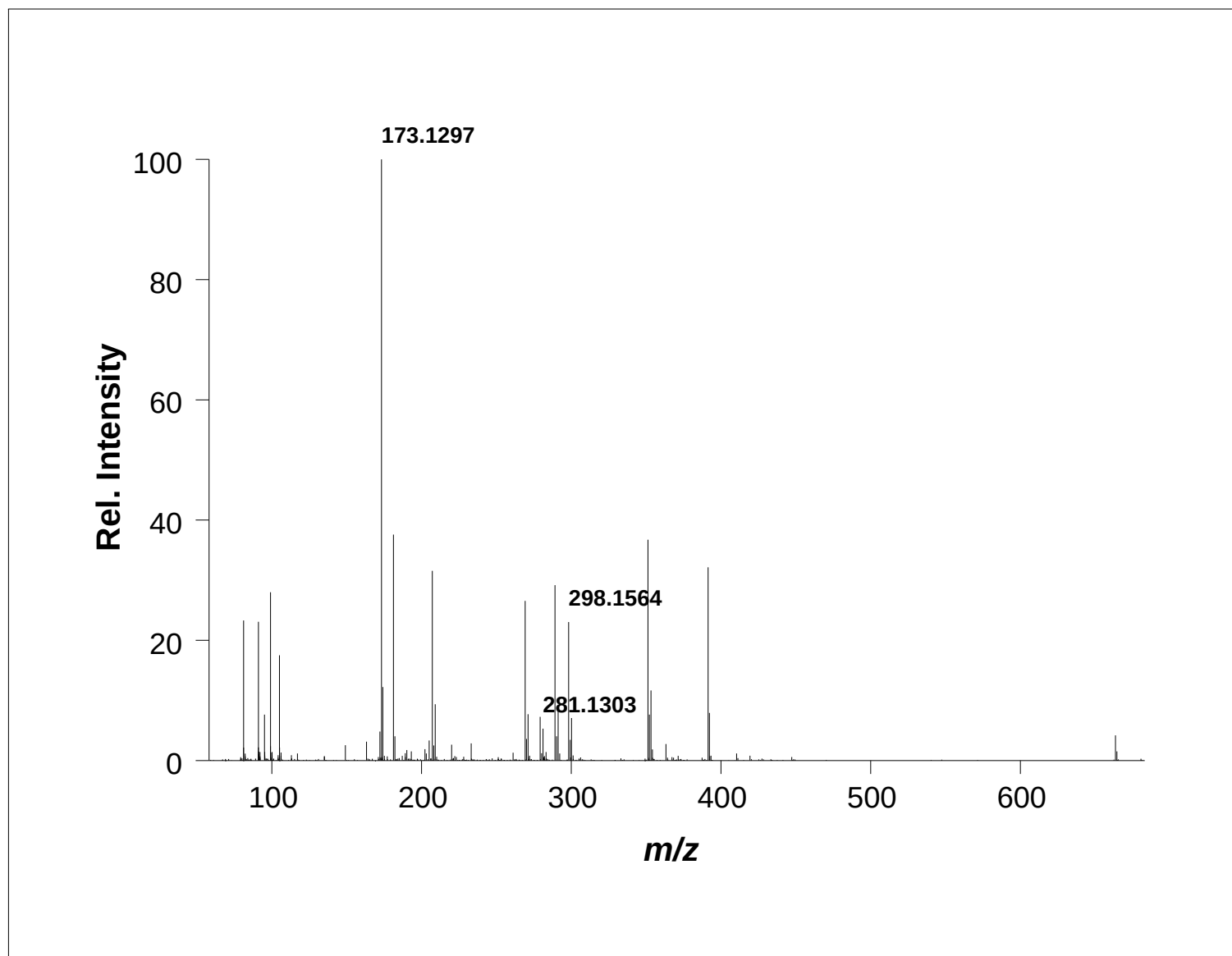
HRMS of Compound 27a+b [( \pm )-(trans-2-benzylcyclohexyl) 2-chloropropanoate]
