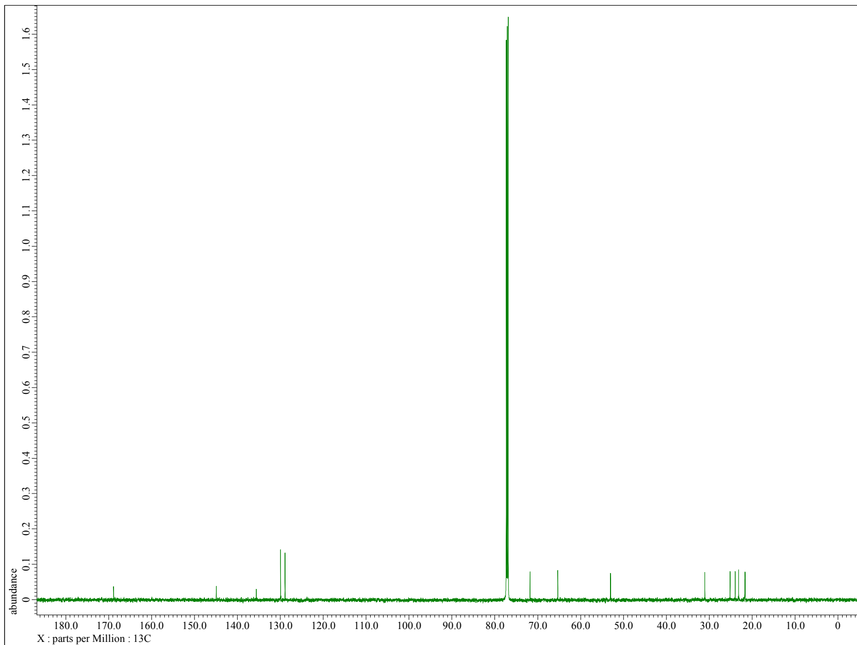
^{13}\text{C} NMR of Compound 26a+b [( \pm )-(trans-2-(p-tolylsulfonyl)cyclohexyl 2-chloropropanoate]
